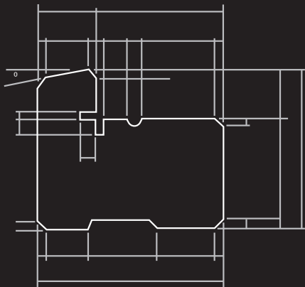
DF-02 56mm x 68mm Head/Jamb
